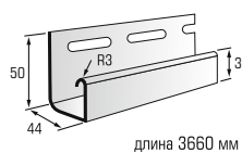
4 J-trim
